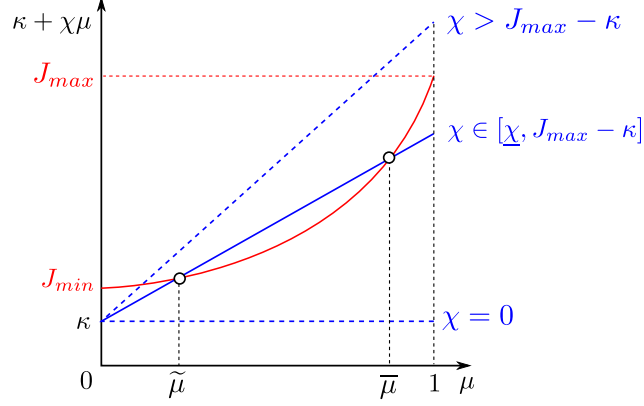
Figure 1. Multiple steady states
